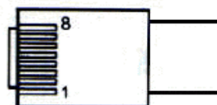
Plug End RJ-45 8 conductor
